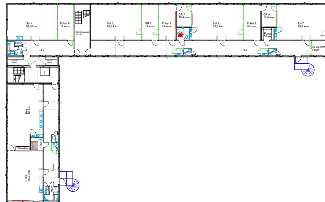
Plan 3
