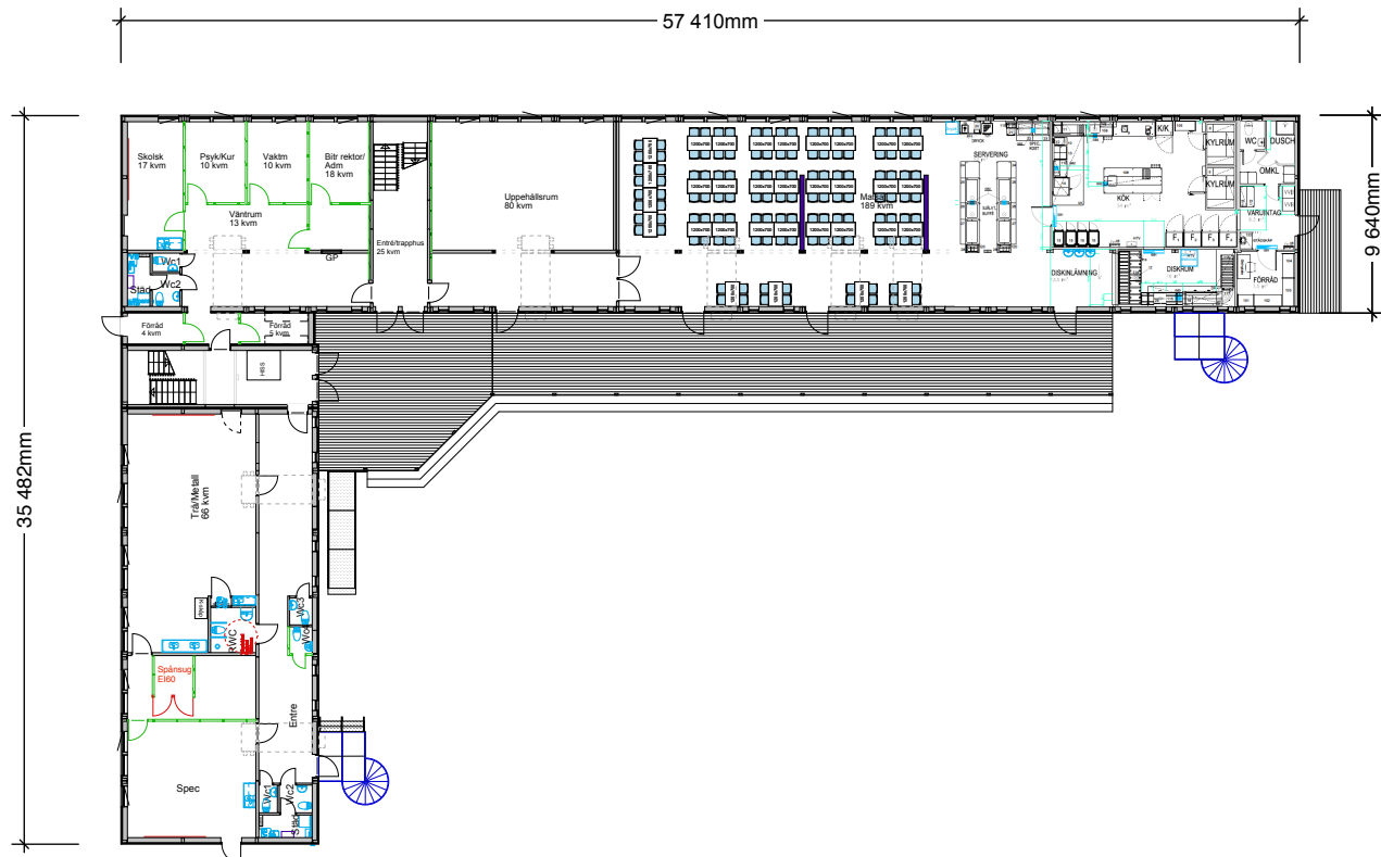
Plan 1
